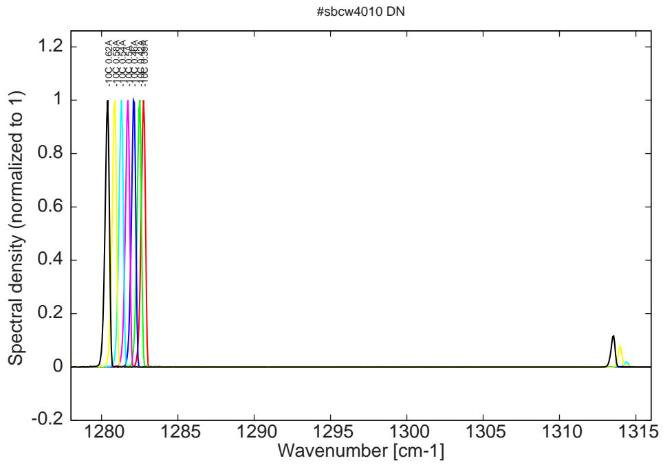
Figure 10: spectra at -10C for various DC currents (monomode up to 0.5A)
