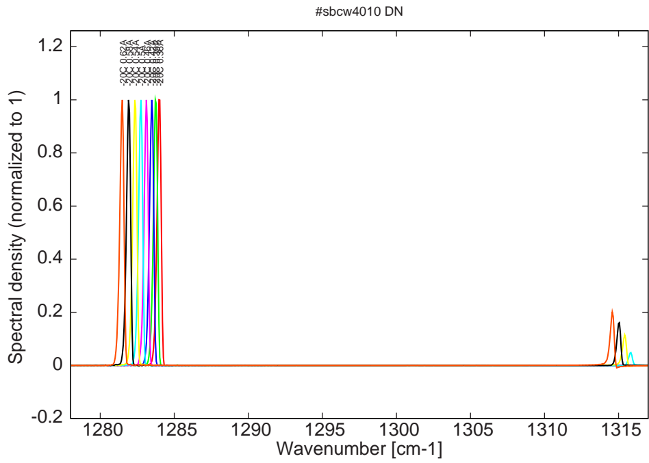
Figure 8: spectra at -20C for various DC currents (monomode up to 0.46A)
