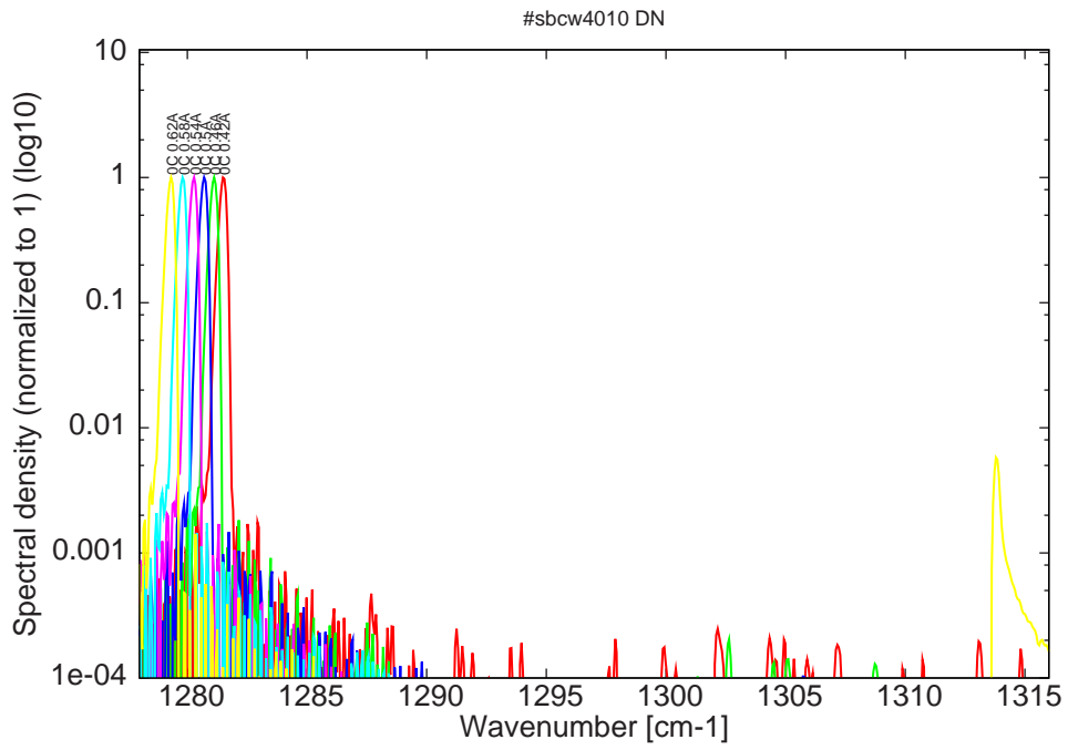
Figure 12: spectra at 0C for various DC currents (monomode up to 0.58A)
