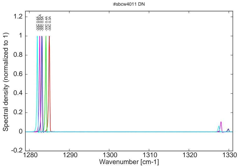
Figure 6: spectra at -30C for various DC currents (monomode up to 0.4A)
