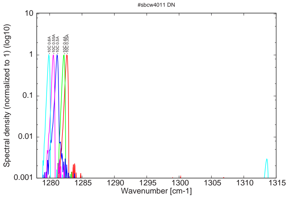
Figure 10: spectra at -10C for various DC currents (monomode up to 0.55A)
