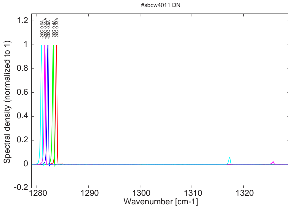
Figure 8: spectra at -20C for various DC currents (monomode up to 0.5A)
