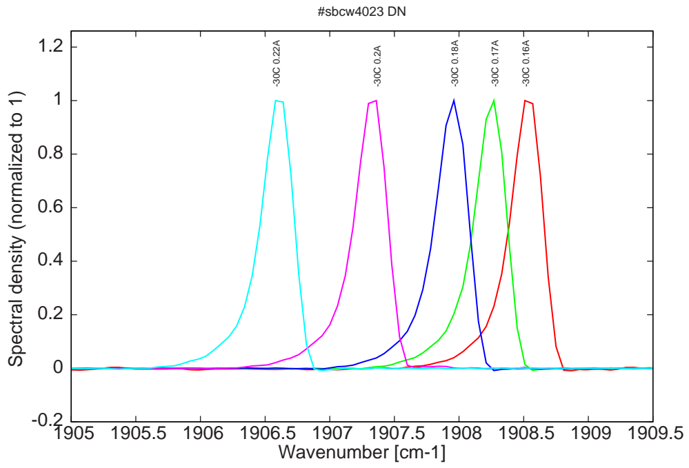
Figure 5: spectra at -30C for various DC currents (monomode with mode jumping for I > 0.18A )
