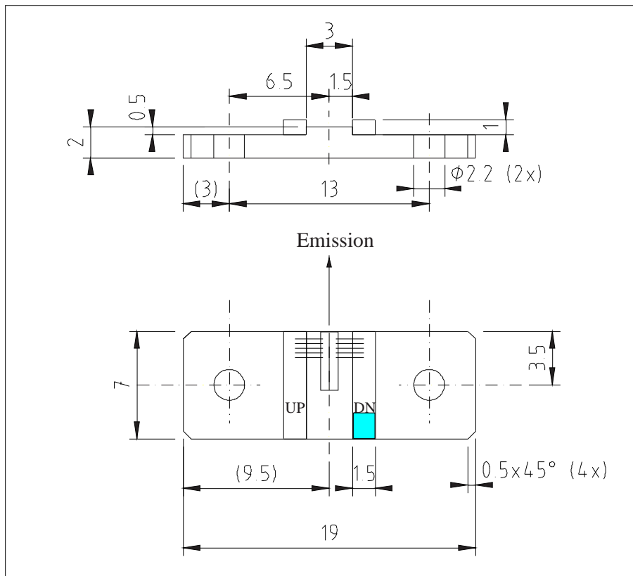
Figure 1: Support mounting for #sbcw4023 DN (please note that the laser is connected to the DN pad drawn in blue)
