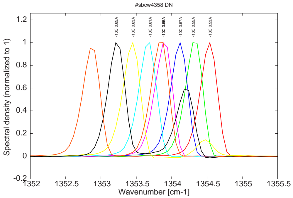
Figure 10: spectra at -10C for various DC currents (monomode up to 0.61A, then becomes bimode)
