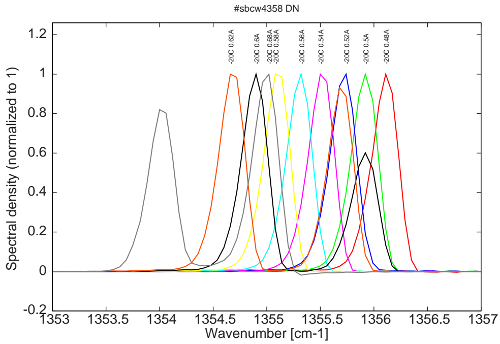
Figure 8: spectra at -20C for various DC currents (monomode up to 0.58A, then becomes bimode)
