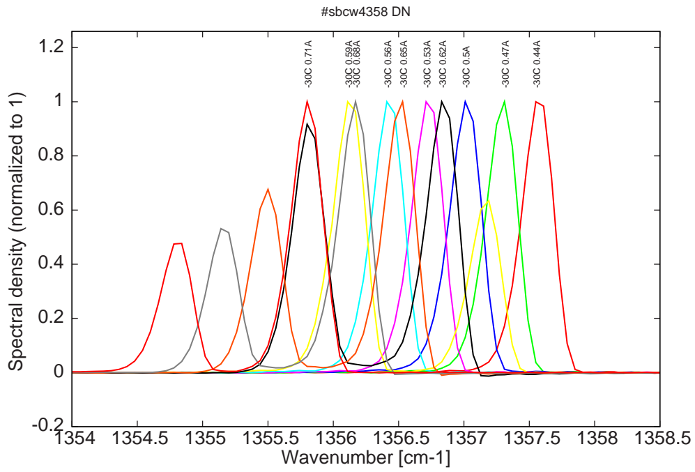
Figure 6: spectra at -30C for various DC currents (monomode up to 0.56A, then becomes bimode)
