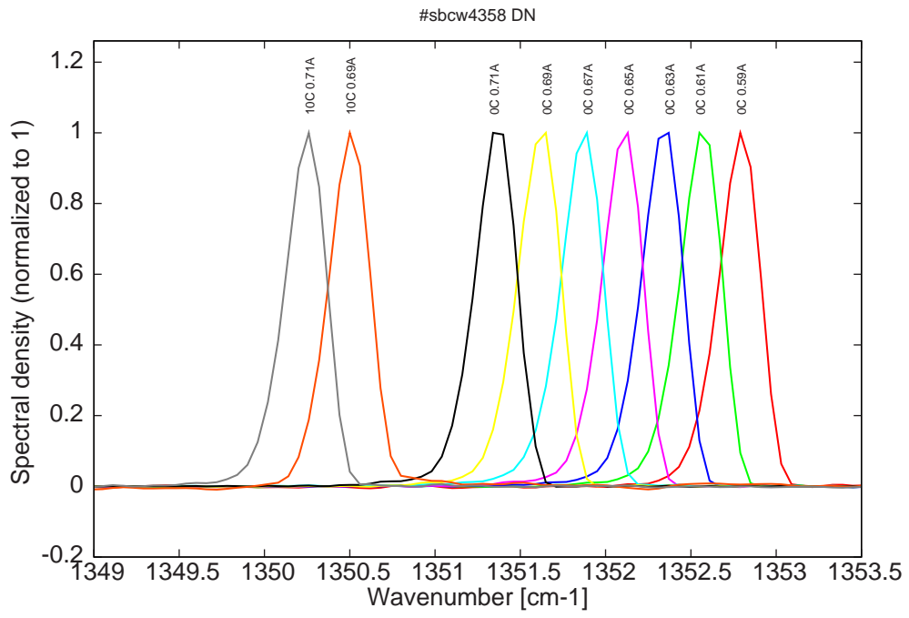
Figure 12: spectra at 0C and 10C for various DC currents (all monomode)
