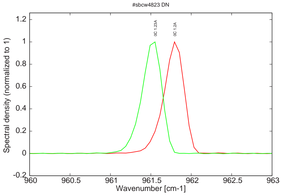
Figure 5: spectra at 0C for various DC currents (all monomode on mode 2, see Fig. 2 & 3)
