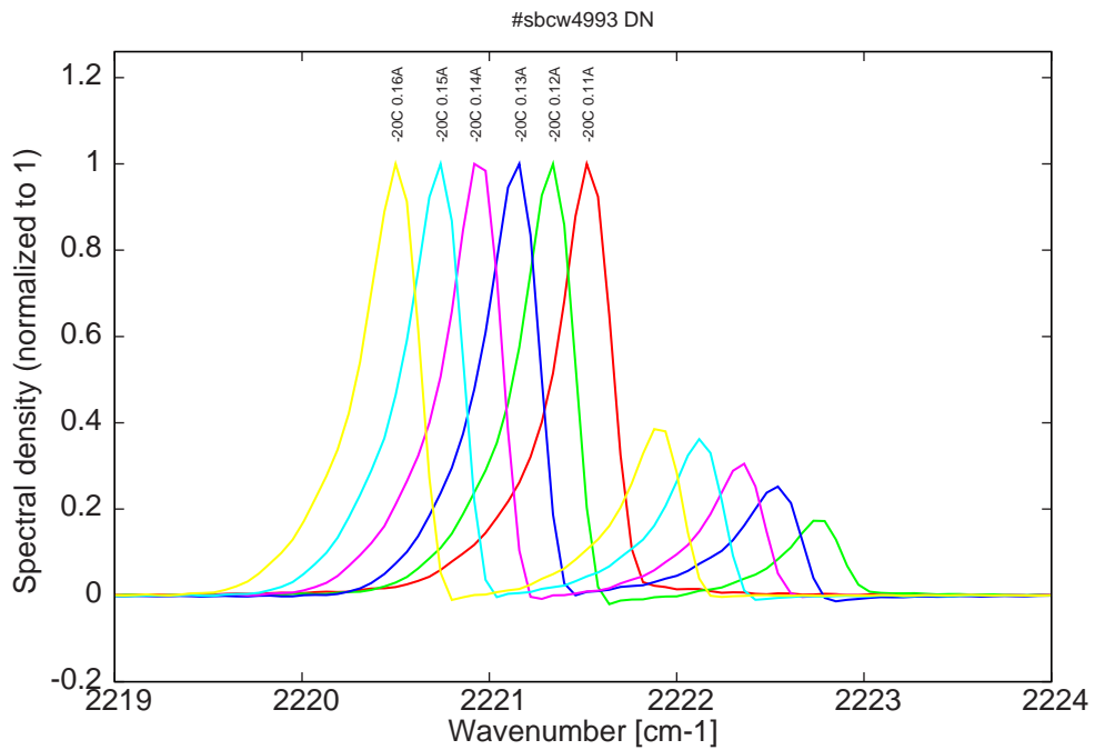
Figure 7: spectra at -20C for various DC currents (monomode on mode 1 up to 0.11A (threshold), then bimode, see Fig. 2 & 3)
