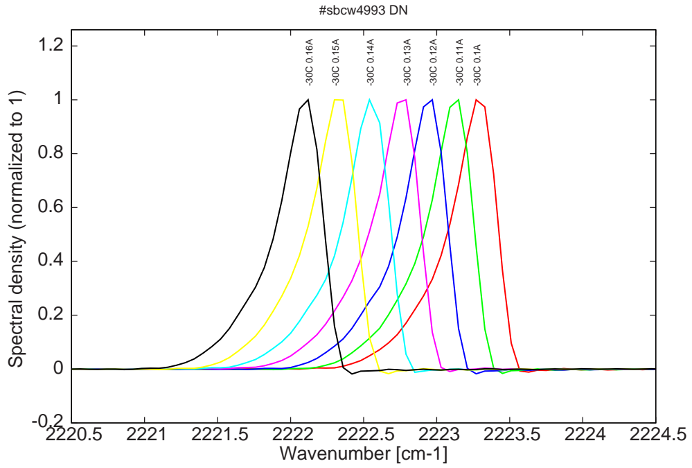
Figure 6: spectra at -30C for various DC currents (monomode on mode 1, see Fig. 2 & 3)
