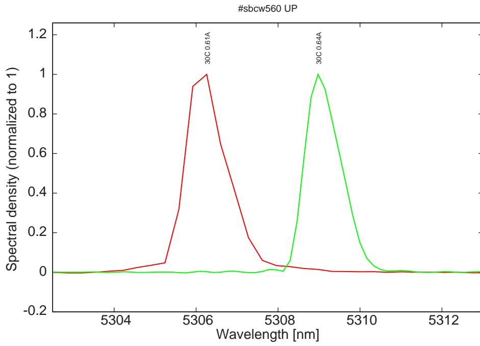
Figure 16: spectra at 30C for various DC currents
