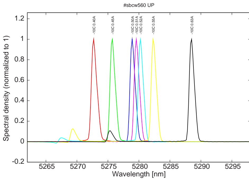
Figure 11: spectra at -10C for various DC currents (monomode up to 0.51A)
