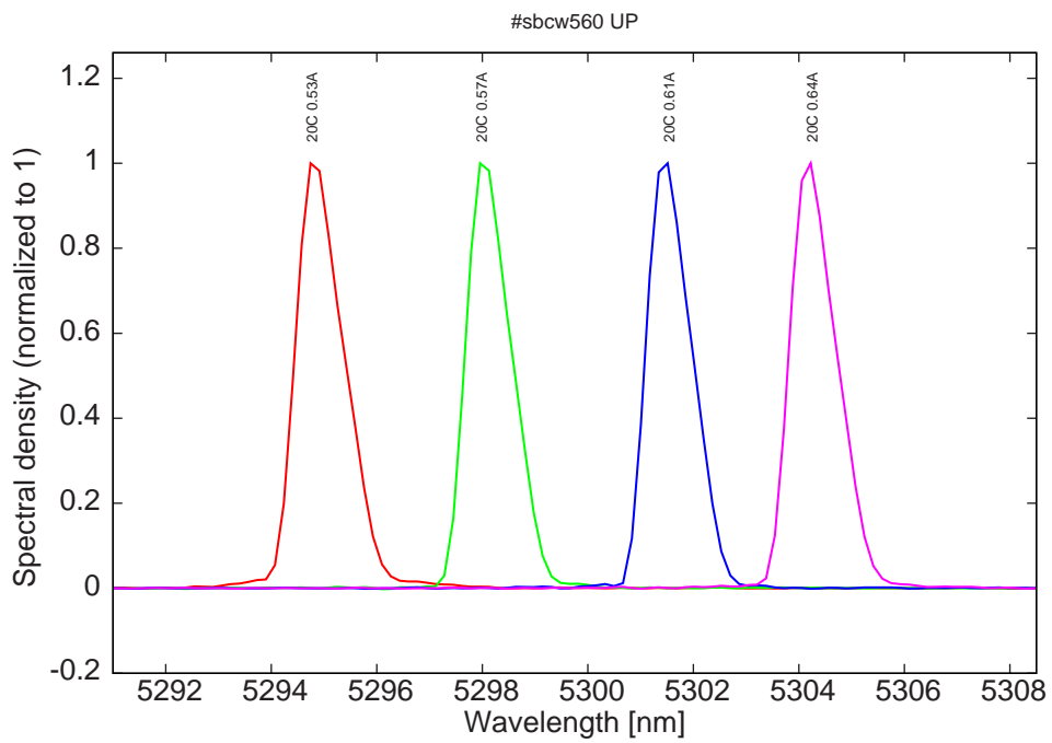
Figure 15: spectra at 20C for various DC currents
