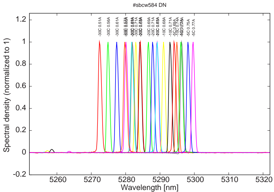
Figure 6: spectra at -30C, -20C, -10C and -5C for various DC currents
