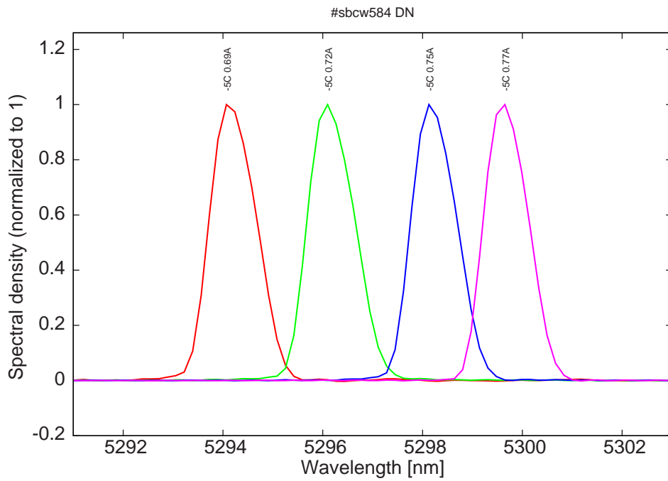
Figure 12: spectra at -5C for various DC currents
