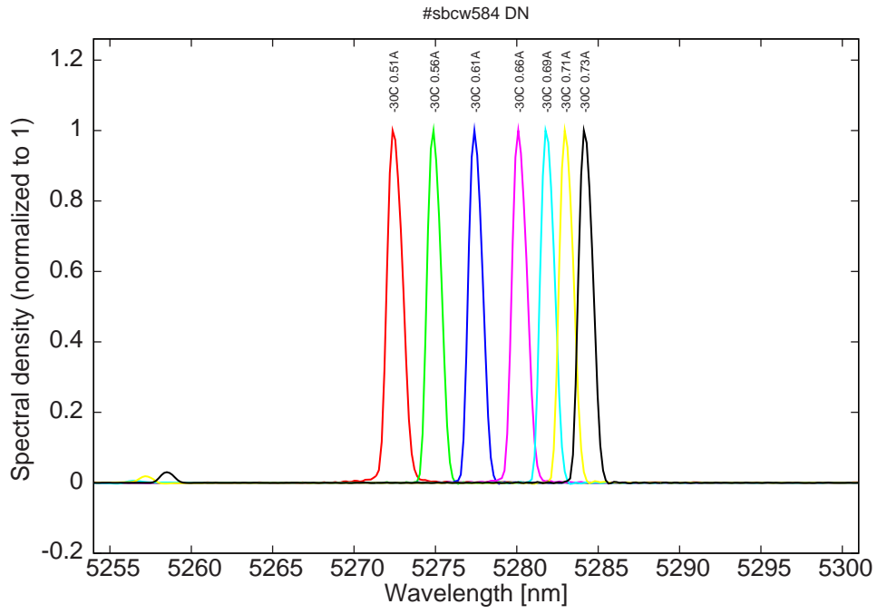
Figure 7: spectra at -30C for various DC currents (monomode up to 0.66A)
