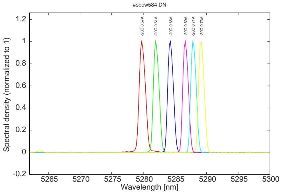
Figure 9: spectra at -20C for various DC currents (monomode up to 0.71A)
