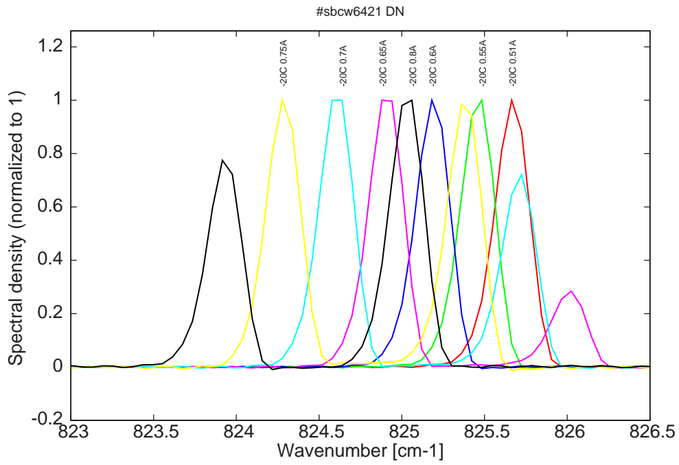
Figure 6: spectra at -20C for various DC currents (monomode up to 0.6A, then becomes bimode)
