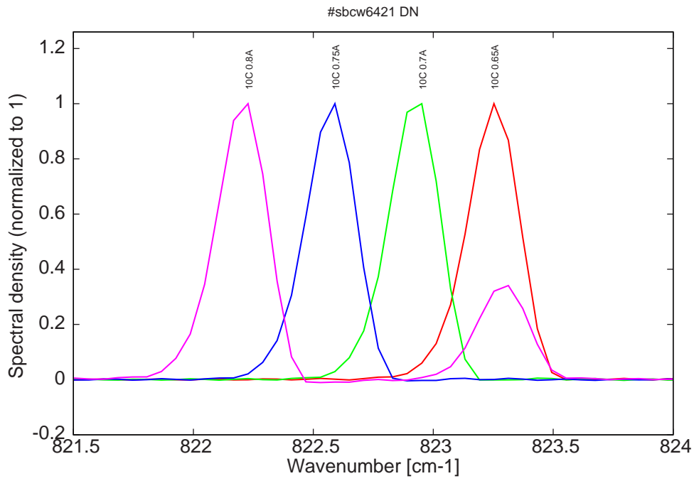
Figure 12: spectra at 10C for various DC currents (monomode up to 0.75A, then becomes bimode)
