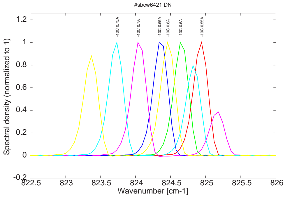
Figure 8: spectra at -10C for various DC currents (monomode up to 0.65A, then becomes bimode)
