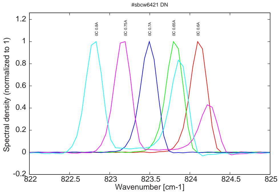
Figure 10: spectra at 0C for various DC currents (monomode up to 0.7A, then becomes bimode)
