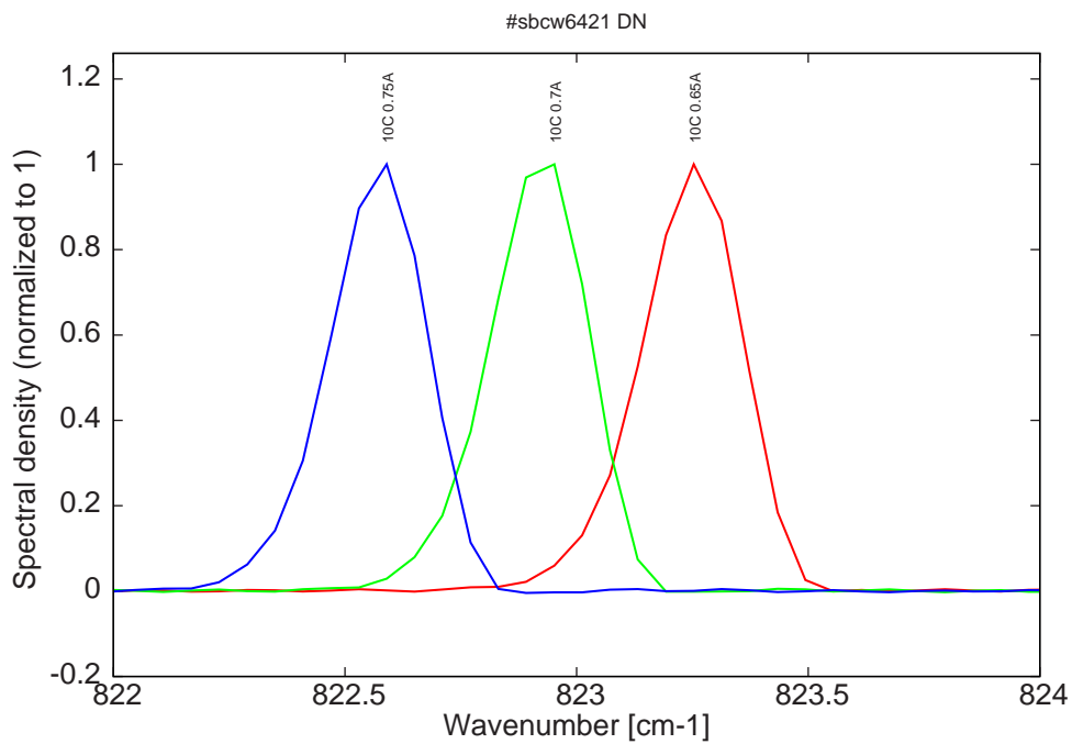
Figure 13: spectra at 10C for various DC currents (monomode range)
