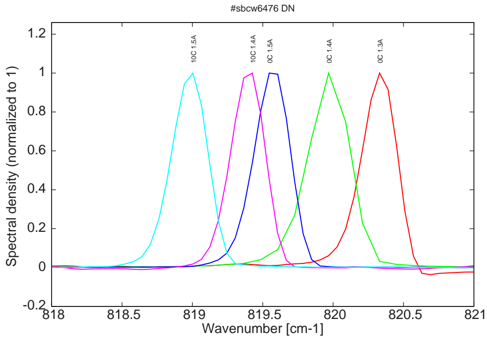
Figure 10: spectra between 0C and 20C for various DC currents (all monomode)
