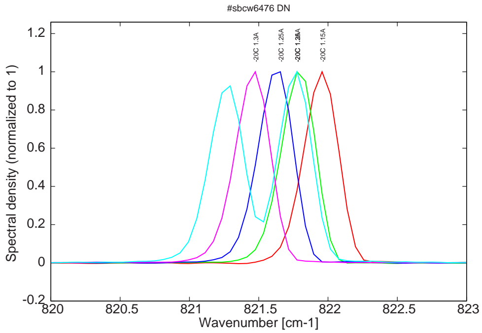
Figure 6: spectra at -20C for various DC currents (monomode up to 1.3A, then becomes bimode)
