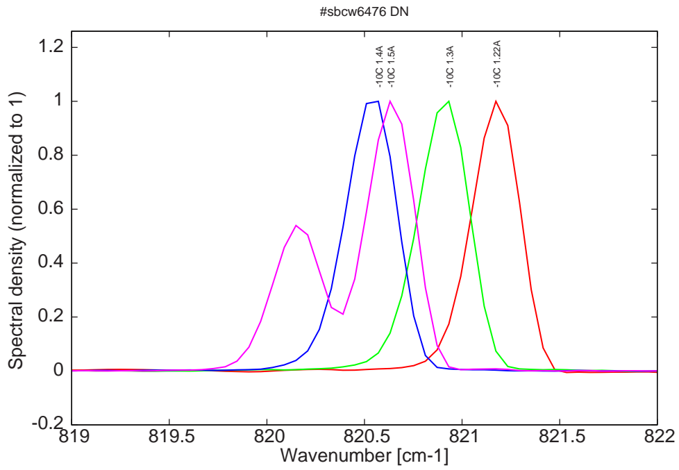
Figure 8: spectra at -10C for various DC currents (monomode up to 1.4A, then becomes bimode)
