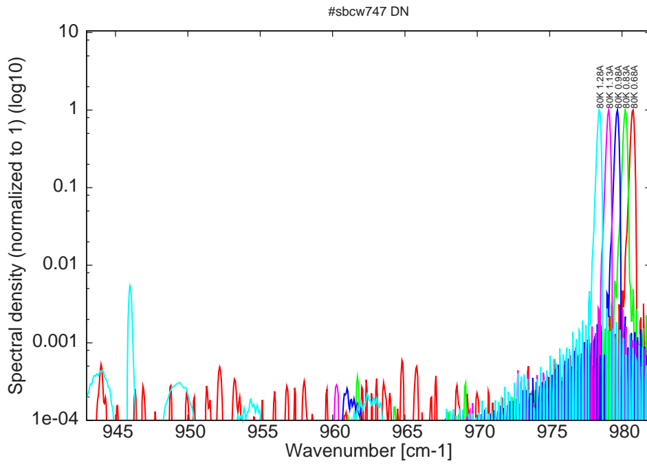
Figure 6: spectra at 80K for various DC currents (become bimode for I > 1.13A )
