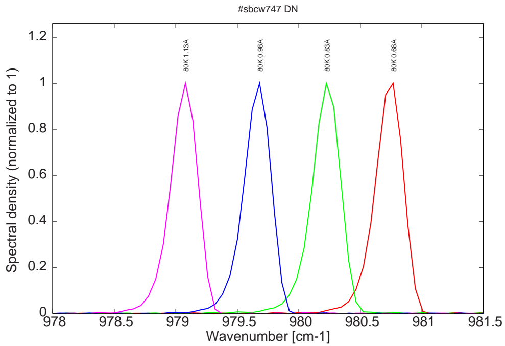
Figure 7: spectra at 80K for various DC currents (monomode range)
