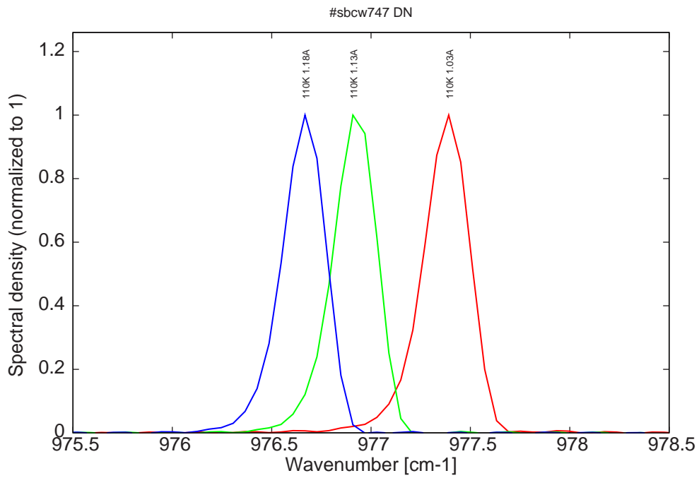
Figure 11: spectra at 110K for various DC currents (monomode range)
