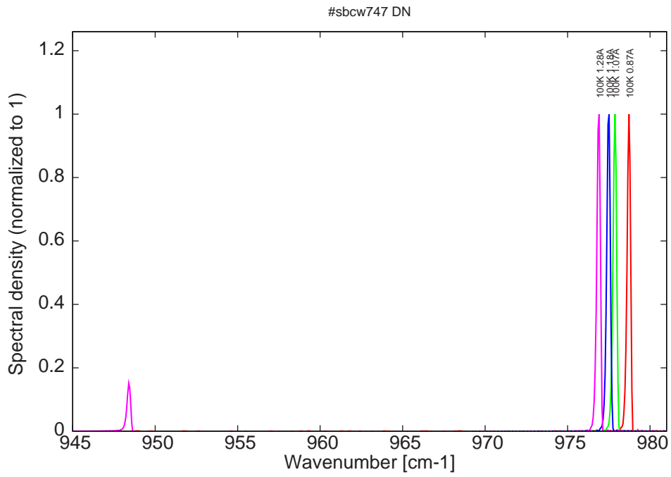
Figure 8: spectra at 100K for various DC currents (become bimode for I > 1.18\text{A} )
