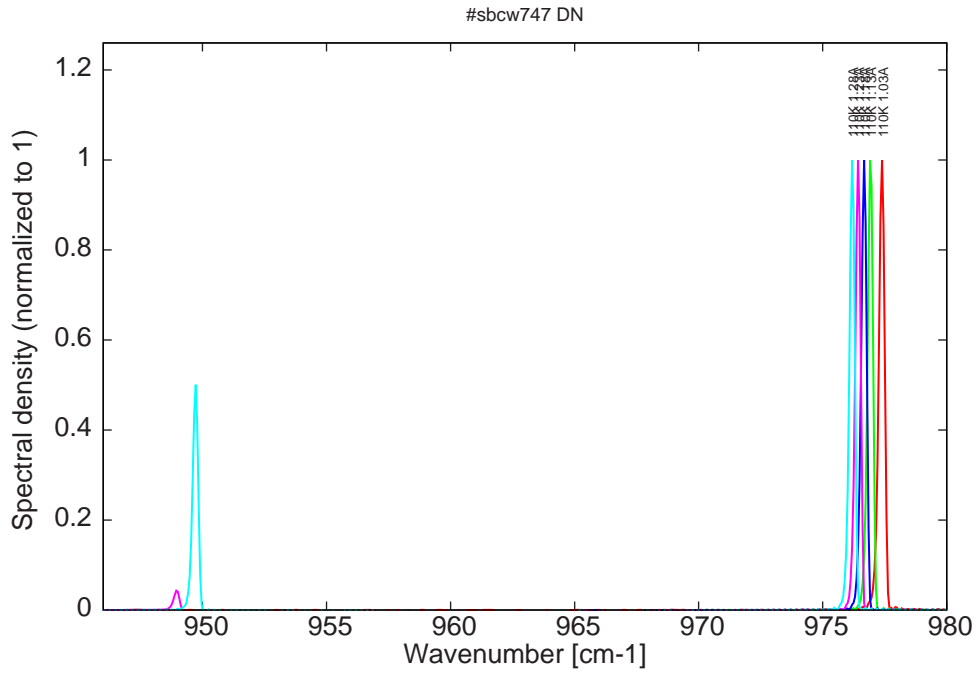
Figure 10: spectra at 110K for various DC currents (become bimode for I > 1.18A )
