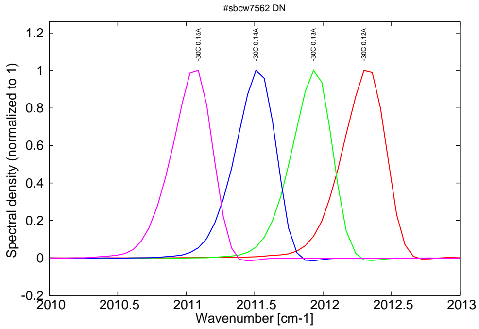
Figure 5: spectra at -30C for various DC currents (monomode on mode 1, see Fig. 2 & 3)
