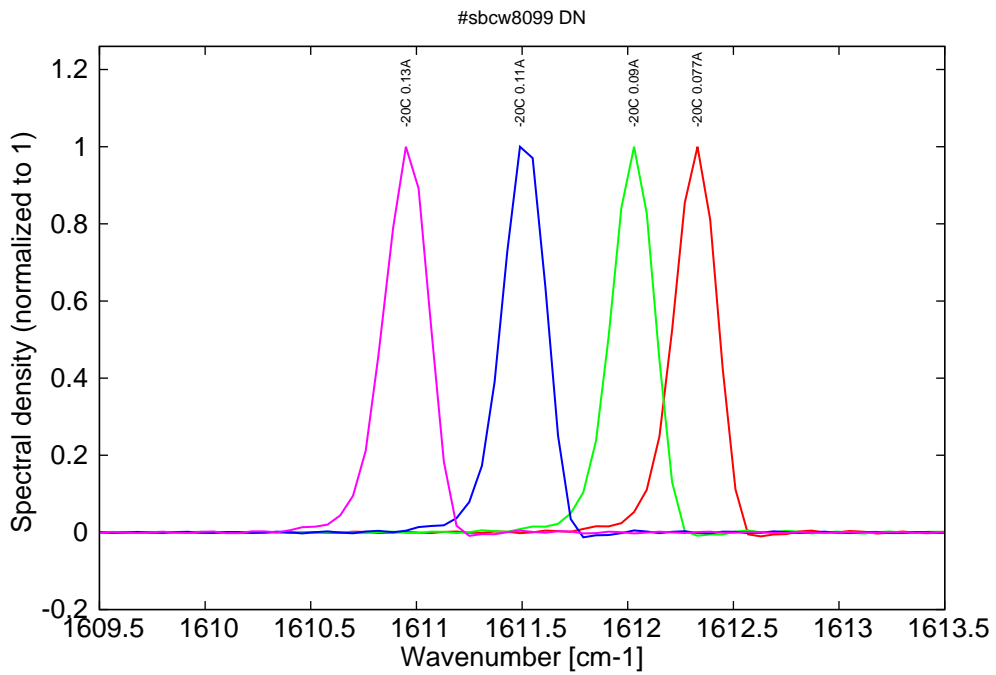
Figure 9: spectra at -20C for various DC currents (monomode up to 0.13A, then becomes bimode)
