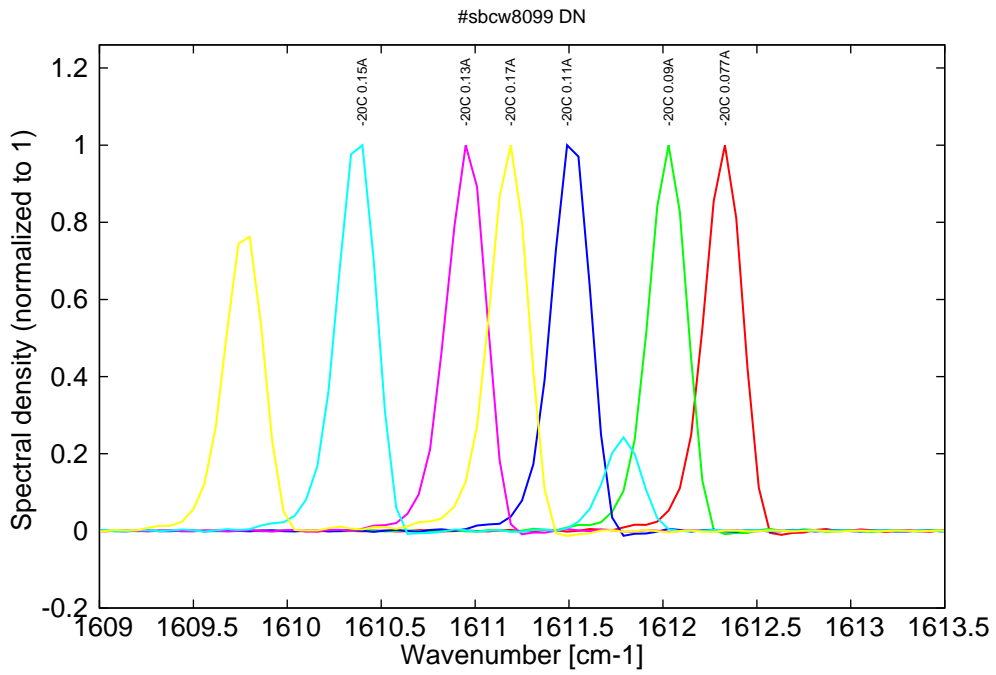
Figure 8: spectra at -20C for various DC currents (monomode up to 0.13A, then becomes bimode)
