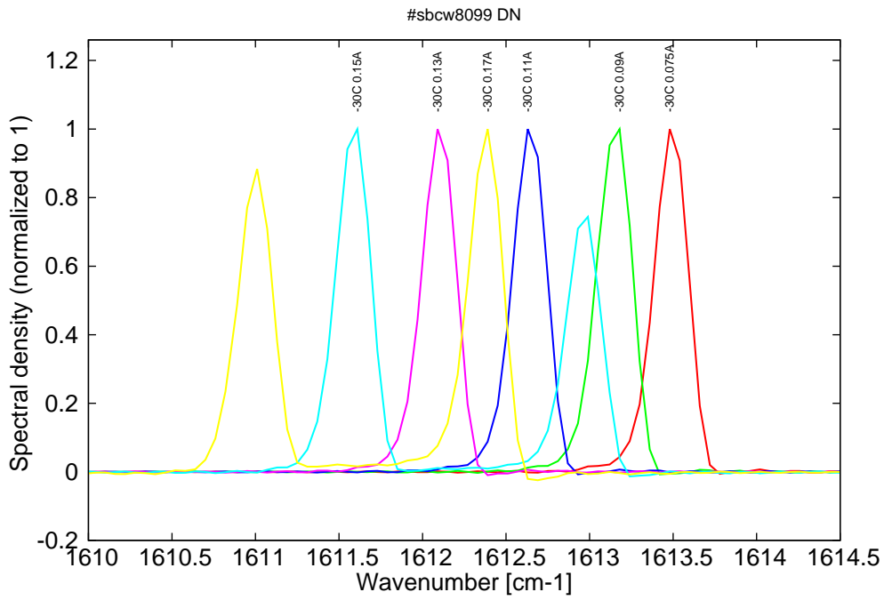
Figure 6: spectra at -30C for various DC currents (monomode up to 0.13A, then becomes bimode)
