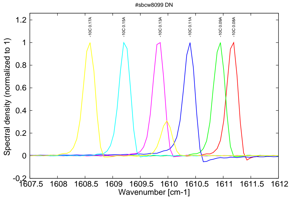
Figure 10: spectra at -10C for various DC currents (monomode up to 0.15A, then becomes bimode)
