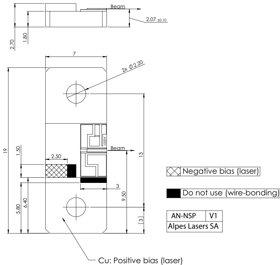
Figure 1: Mechanical and electrical interface for #sbcw8117 DN
