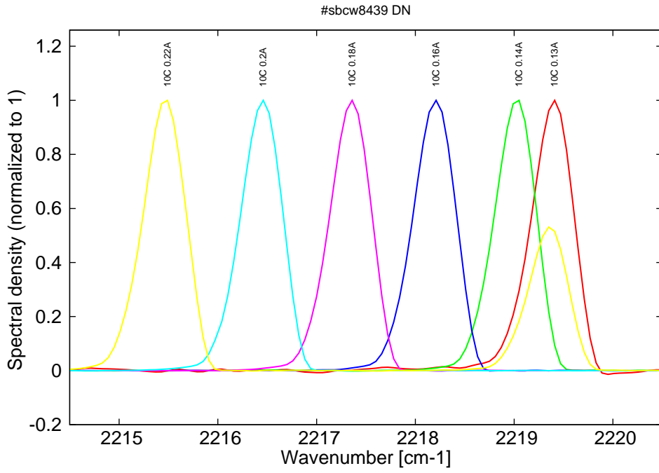
Figure 14: spectra at 10C for various DC currents (monomode up to 0.2A, then becomes bimode)
