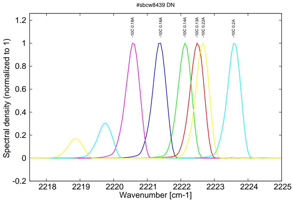
Figure 10: spectra at -10C for various DC currents (monomode up to 0.18A, then becomes bimode)
