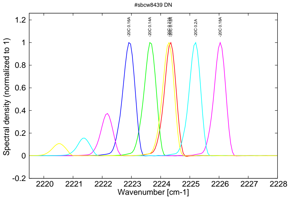
Figure 8: spectra at -20C for various DC currents (monomode up to 0.16A, then becomes bimode)
