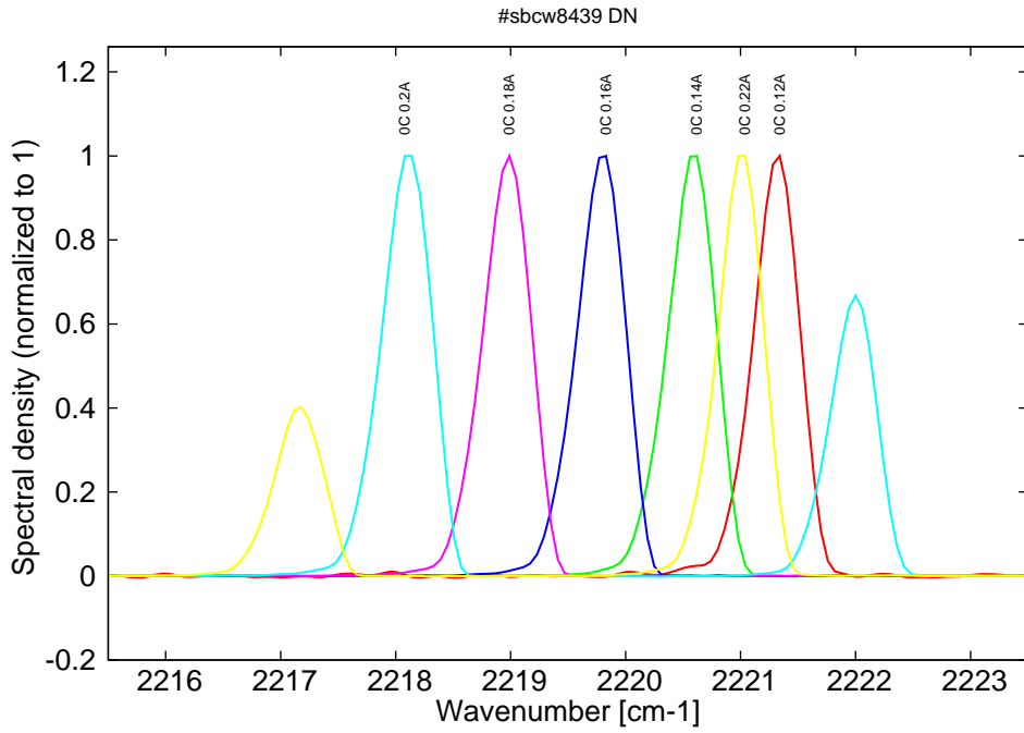
Figure 12: spectra at 0C for various DC currents (monomode up to 0.18A, then becomes bimode)
