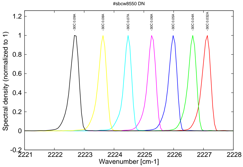
Figure 5: spectra at -30C for various DC currents (monomode on mode 1 up to 70mA, then monomode on mode 2, see kink in LIV)
