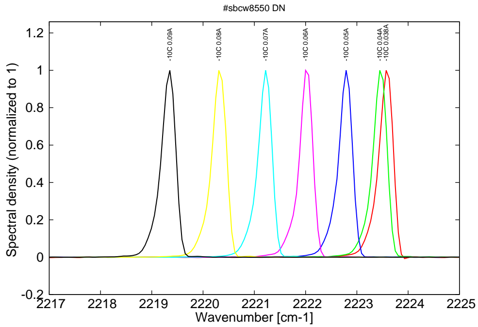
Figure 7: spectra at -10C for various DC currents (monomode on mode 1 up to 50mA, then monomode on mode 2, see kink in LIV)
