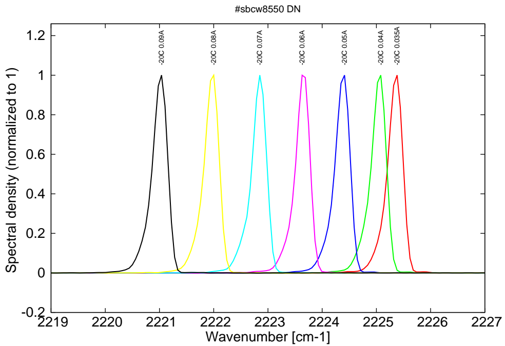
Figure 6: spectra at -20C for various DC currents (monomode on mode 1 up to 60mA, then monomode on mode 2, see kink in LIV)
