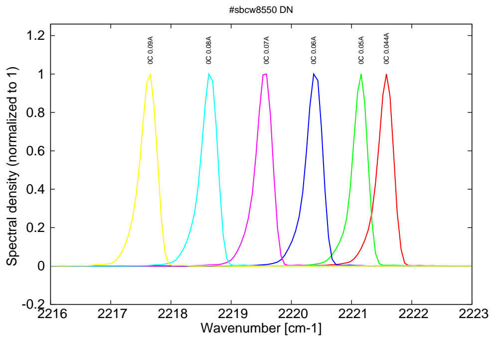
Figure 8: spectra at 0C for various DC currents (monomode on mode 1 up to 44mA, then monomode on mode 2, see kink in LIV)
