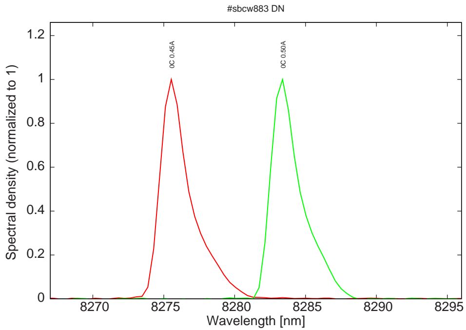
Figure 11: spectra at 0C for various DC currents (all monomode)
