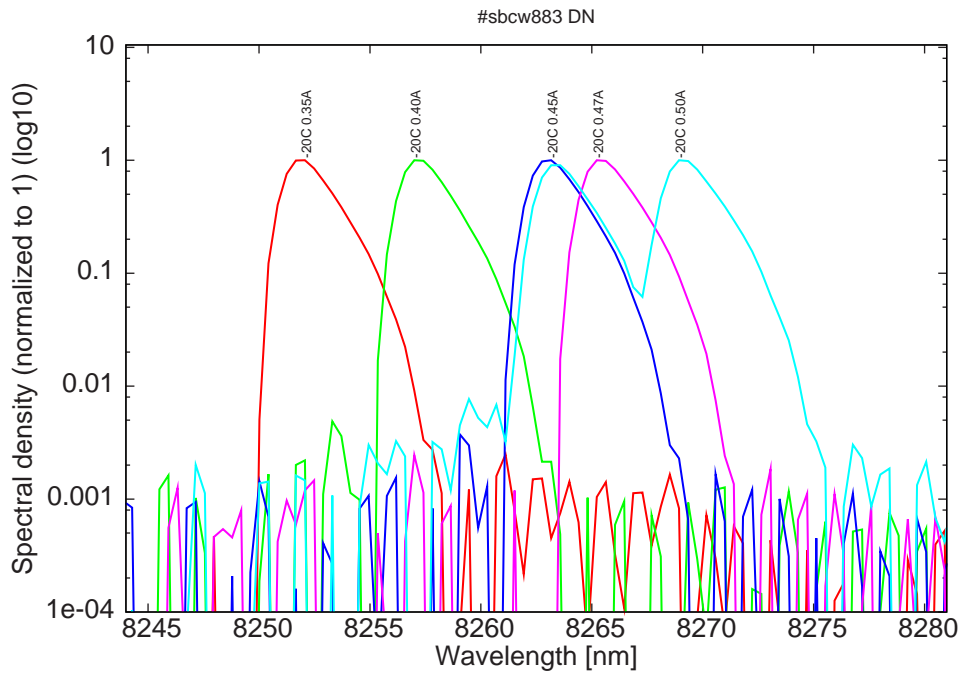
Figure 8: spectra at -20C for various DC currents (monomode up to 0.47A)
