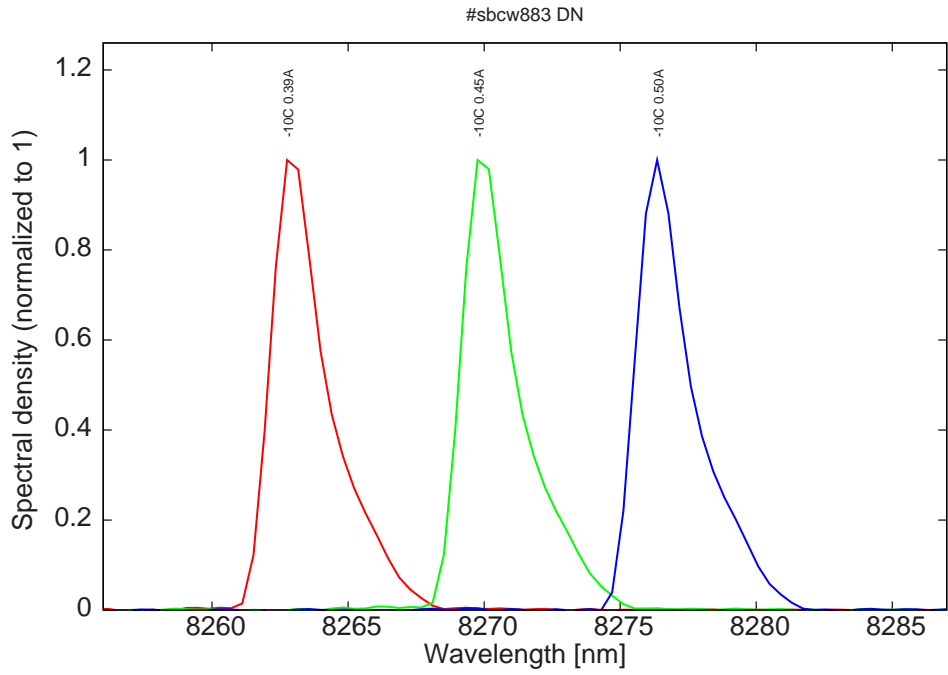
Figure 10: spectra at -10C for various DC currents (all monomode)
