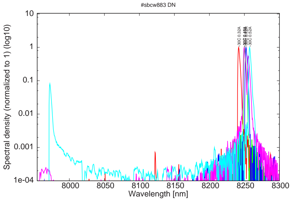
Figure 6: spectra at -30C for various DC currents (monomode up to 0.42A)
