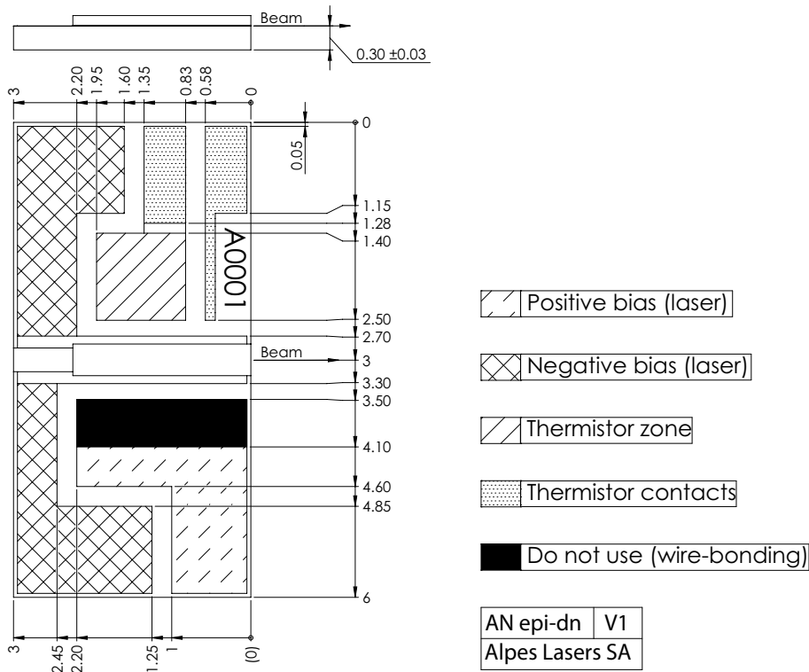
Figure 1: Support mounting for #sbcw9014 DN (please note that AlN submount numbering is A02EZ)
