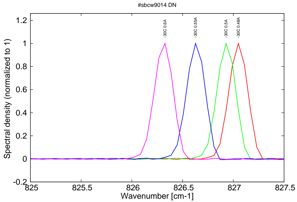
Figure 6: spectra at -30C for various DC currents (monomode up to 0.6A)
