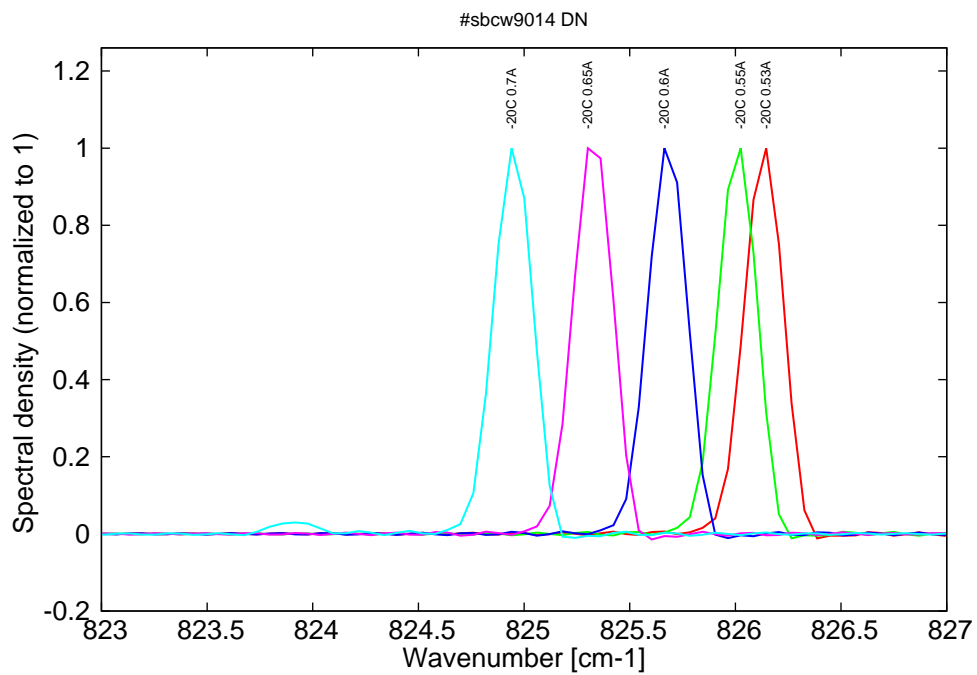
Figure 7: spectra at -20C for various DC currents (monomode up to 0.65A, then becomes bimode)
