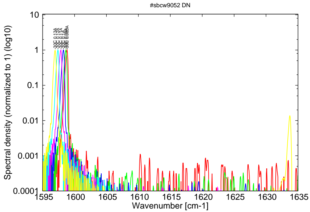
Figure 6: spectra at -30C for various DC currents (monomode up to 0.12A, then becomes bimode)
