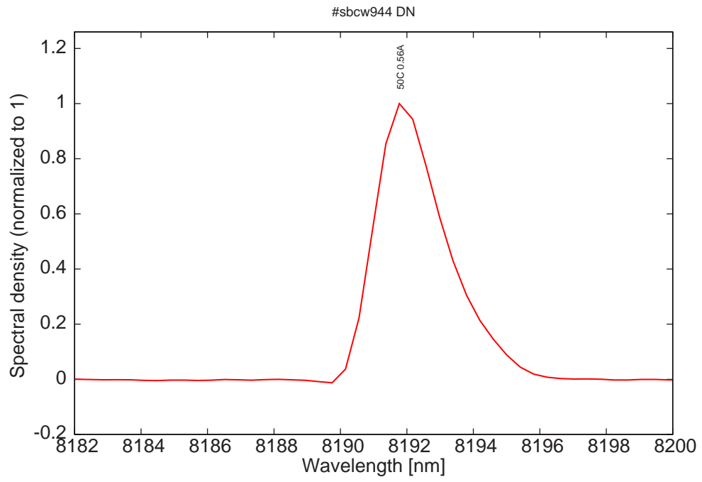
Figure 20: monomode spectrum at 50C and 0.56A
