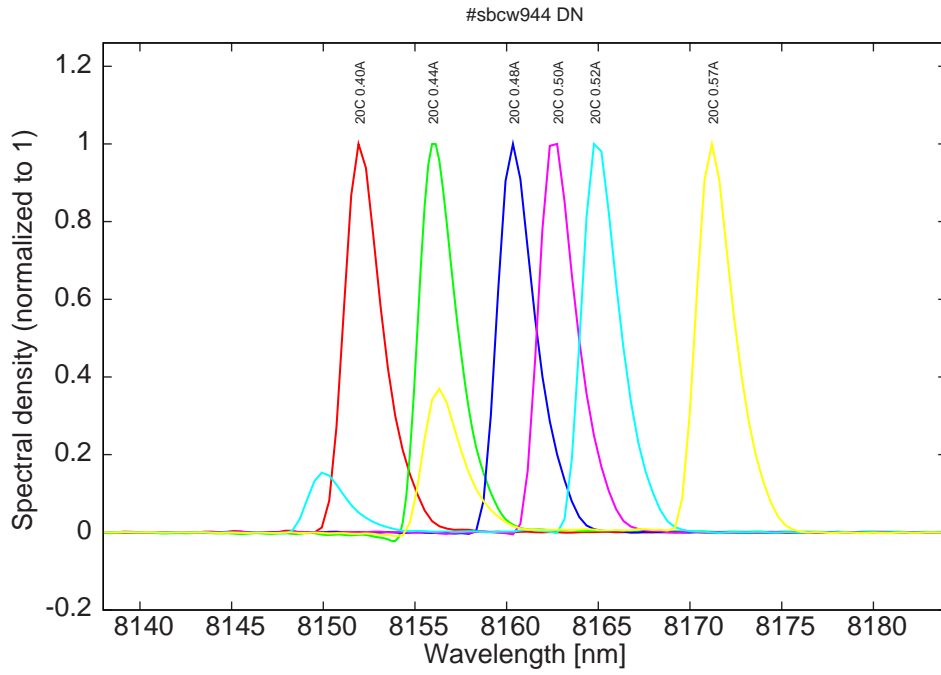
Figure 16: spectra at 20C for various DC currents
