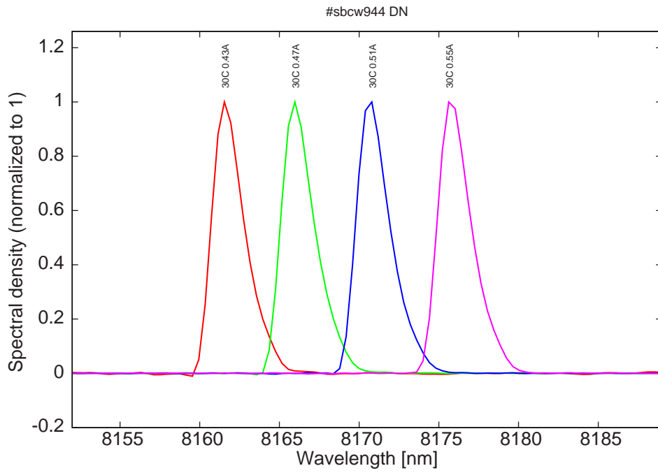
Figure 18: spectra at 30C for various DC currents
