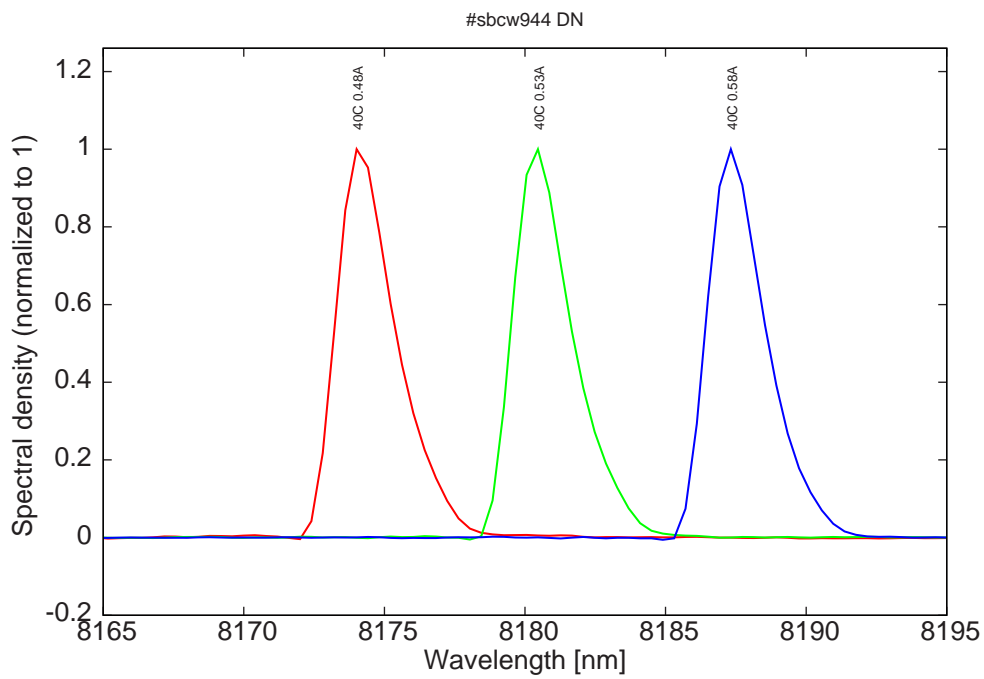
Figure 19: spectra at 40C for various DC currents
