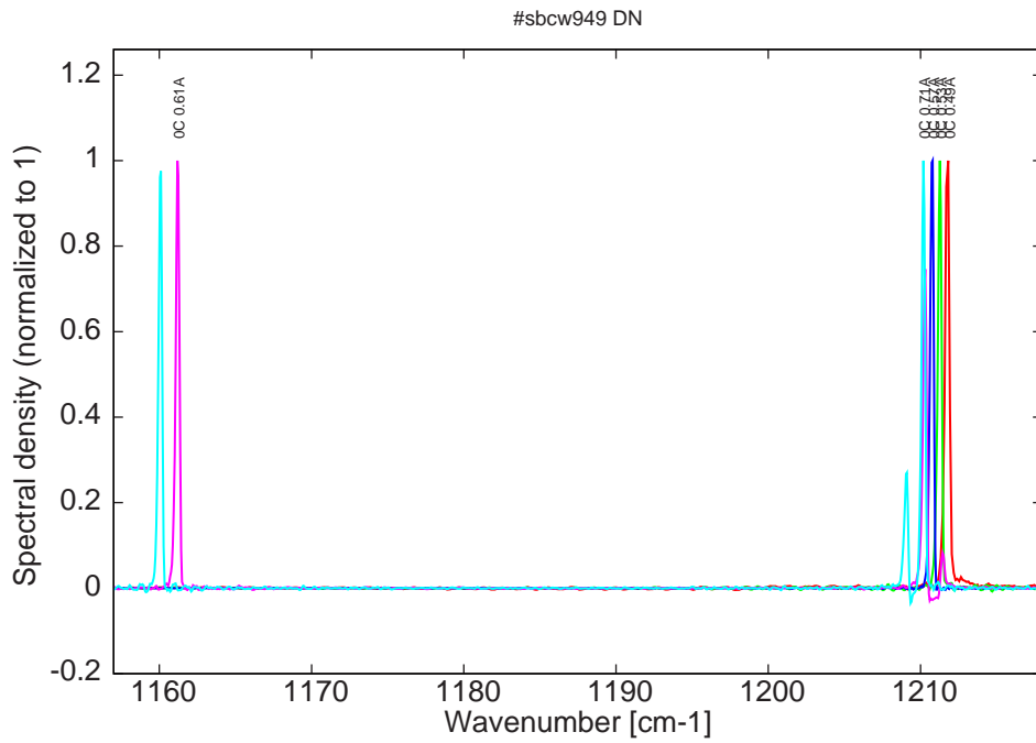
Figure 10: spectra at 0C for various DC currents
