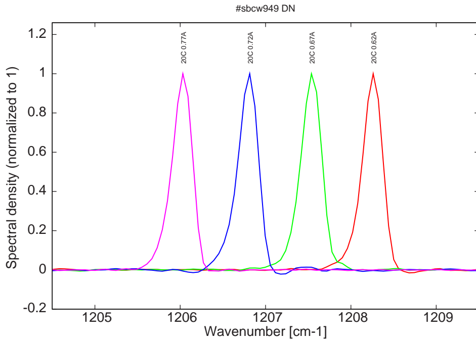
Figure 12: spectra at 20C for various DC currents (all monomode)
