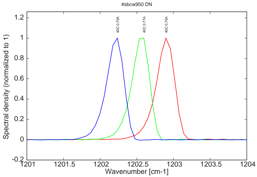
Figure 12: spectra at 40C for various DC currents (all monomode, but with mode jumping compared to spectra at 20C)
