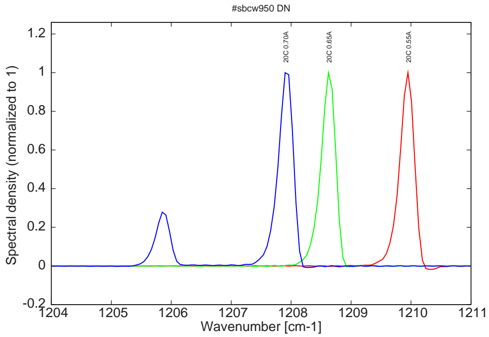
Figure 10: spectra at 20C for various DC currents
