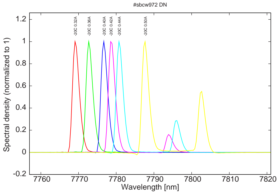
Figure 8: spectra at -20C for various DC currents (monomode up to 0.40A)
