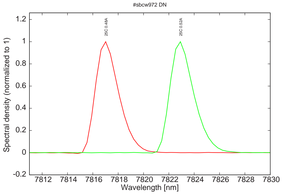
Figure 14: spectra at 25C for various DC currents
