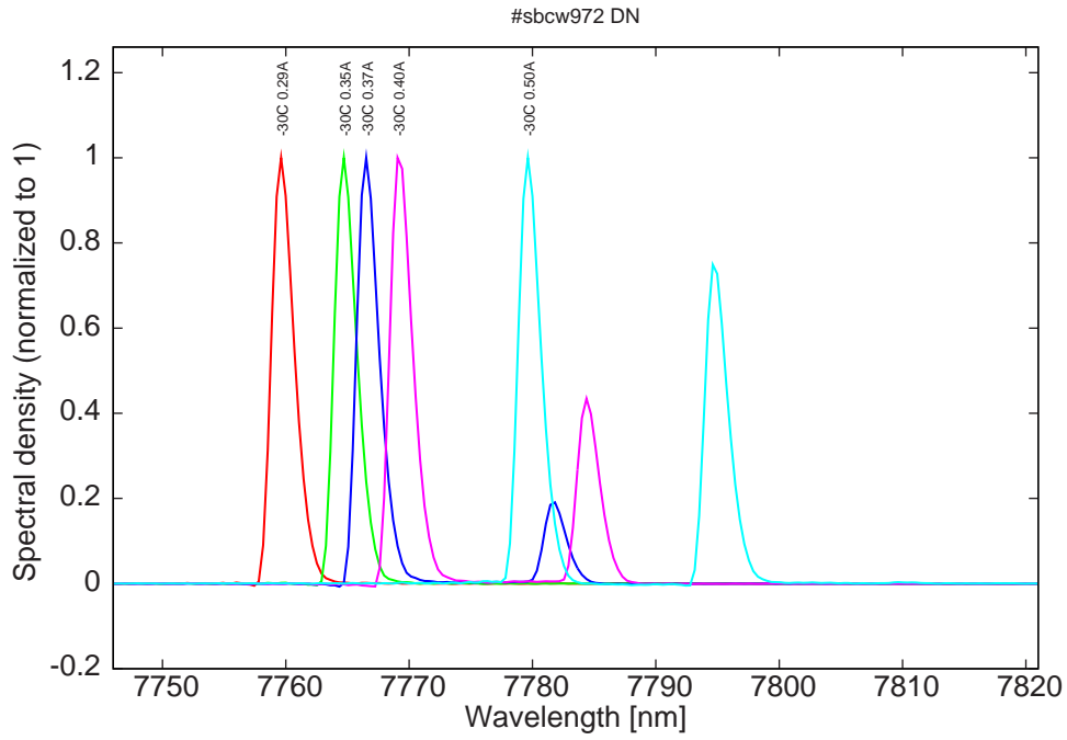
Figure 6: spectra at -30C for various DC currents (monomode up to 0.35A)
