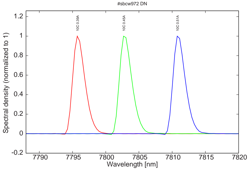
Figure 12: spectra at 10C for various DC currents
