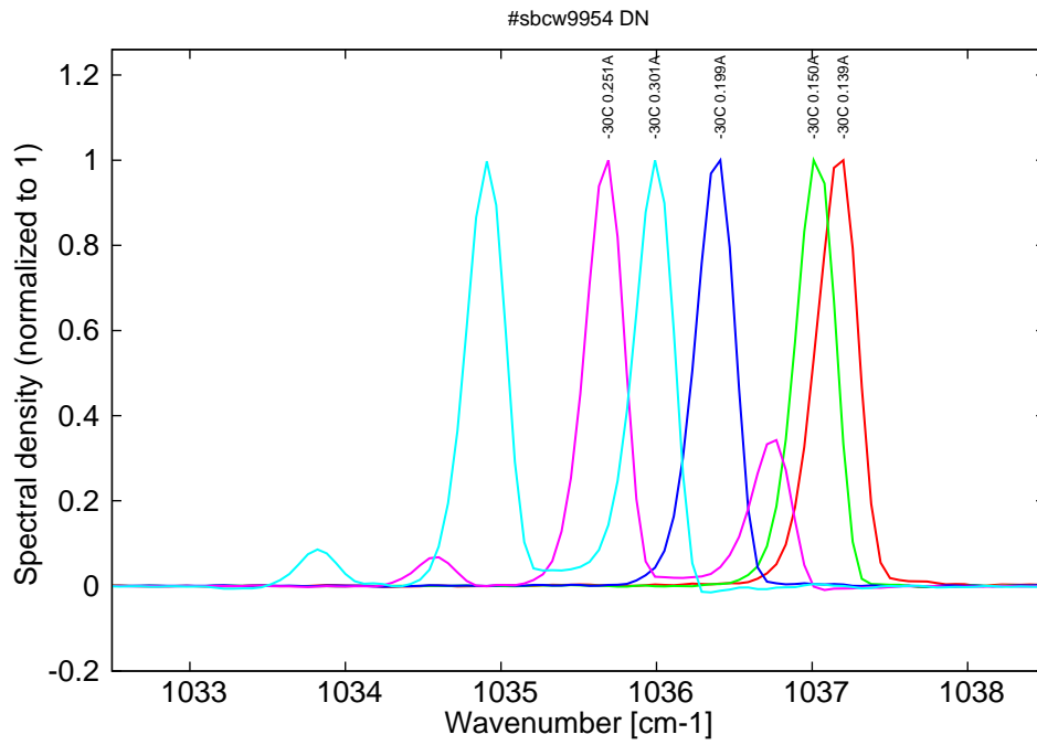
Figure 6: spectra at -30C for various DC currents (monomode up to 0.2A, then becomes multimode)
