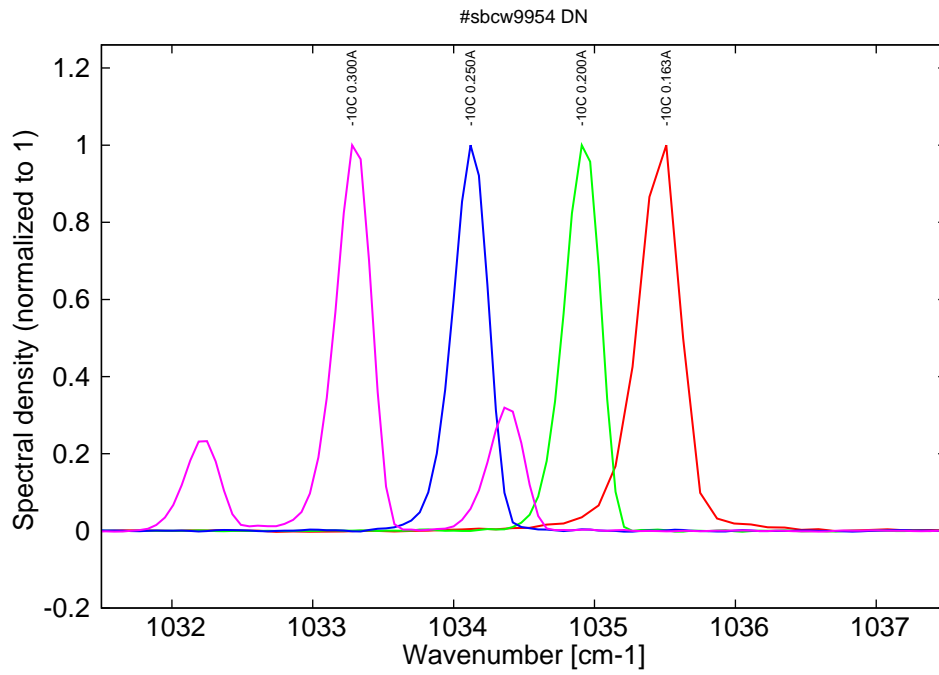
Figure 10: spectra at -10C for various DC currents (monomode up to 0.25A, then becomes multimode)
