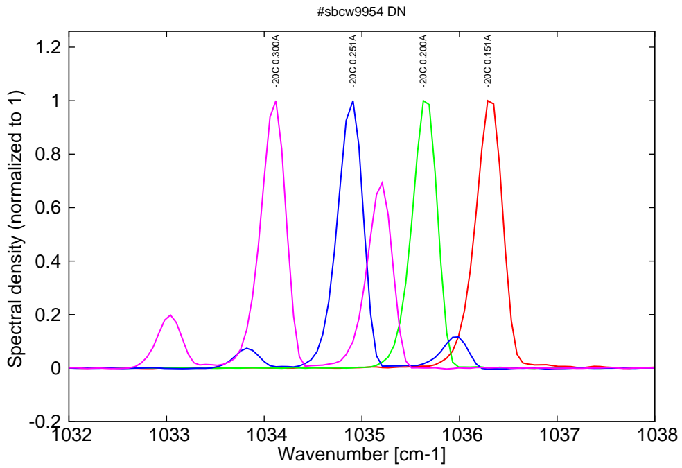
Figure 8: spectra at -20C for various DC currents (monomode up to 0.2A, then becomes multimode)
