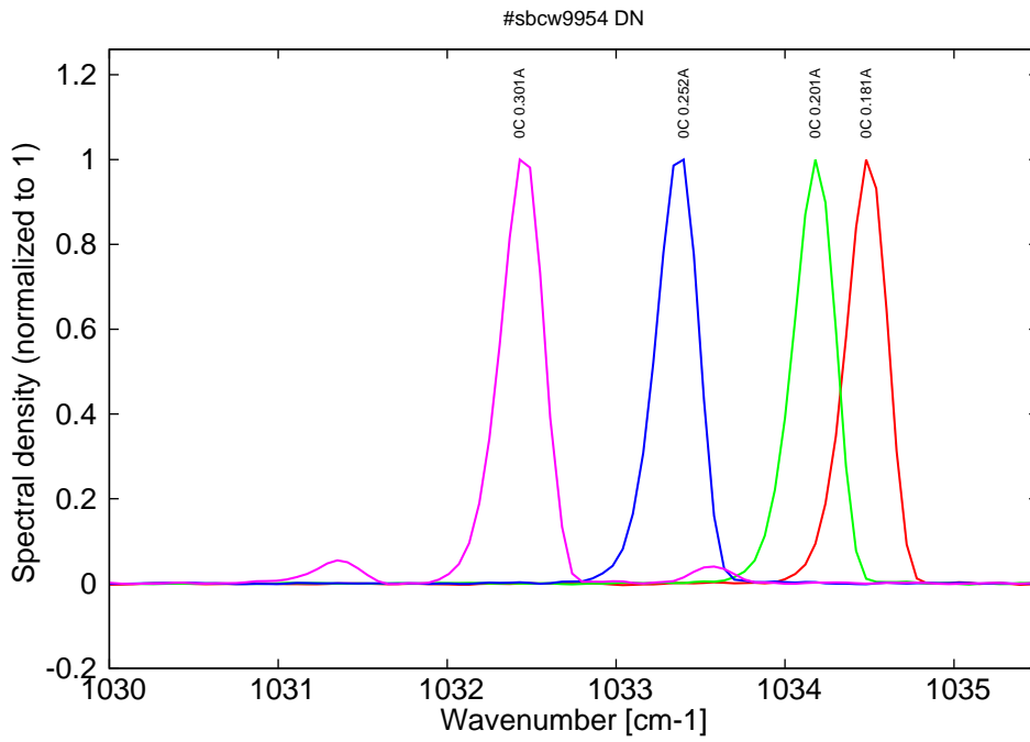
Figure 12: spectra at 0C for various DC currents (monomode up to 0.25A, then becomes multimode)
