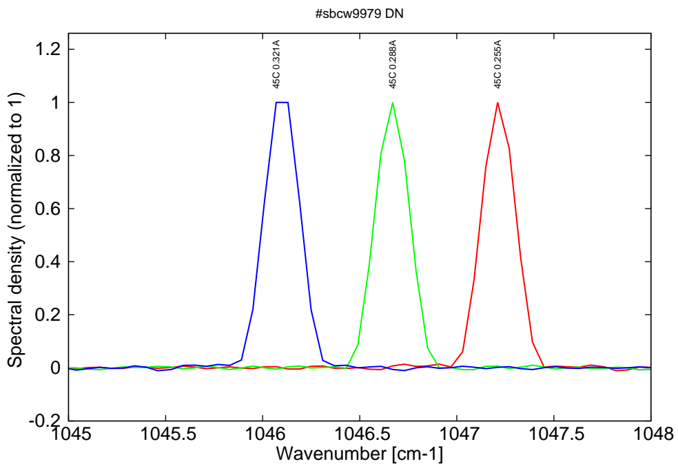
Figure 21: spectra at 45C for various DC currents (monomode range)
