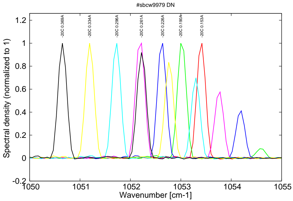
Figure 6: spectra at -20C for various DC currents (monomode up to 0.153A, then becomes bimode)
