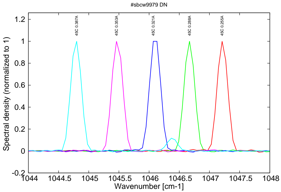
Figure 20: spectra at 45C for various DC currents (monomode up to 0.320A, then becomes bimode)
