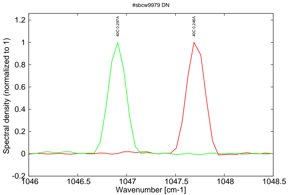
Figure 19: spectra at 40C for various DC currents (monomode range)
