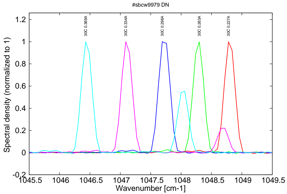
Figure 16: spectra at 30C for various DC currents (monomode up to 0.300A, then becomes bimode)
