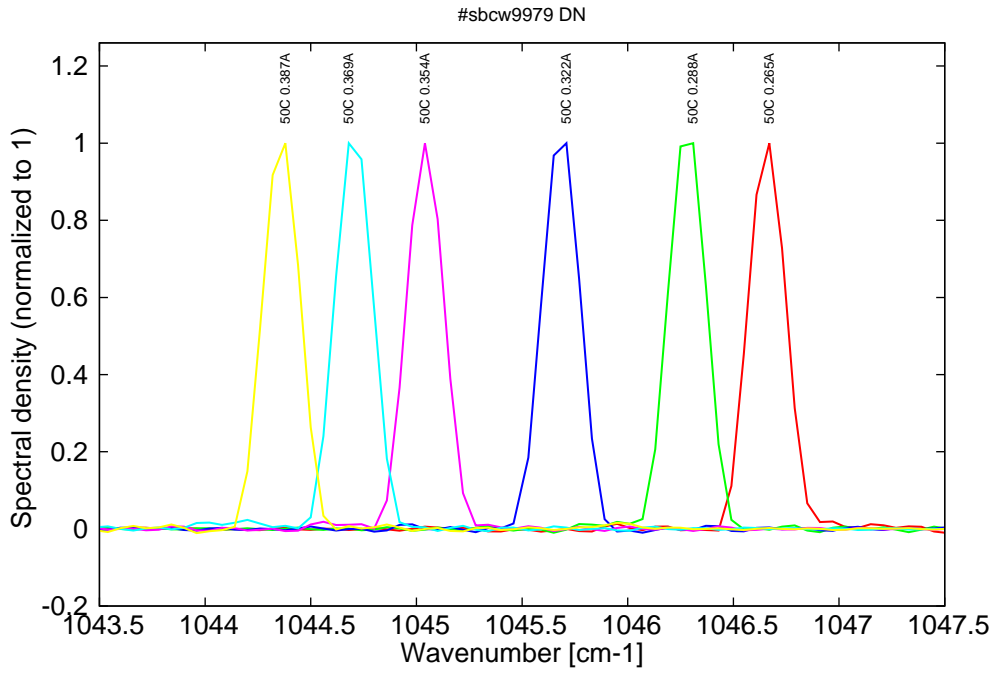
Figure 22: spectra at 50C for various DC currents (monomode up to 0.370A, then becomes bimode)
