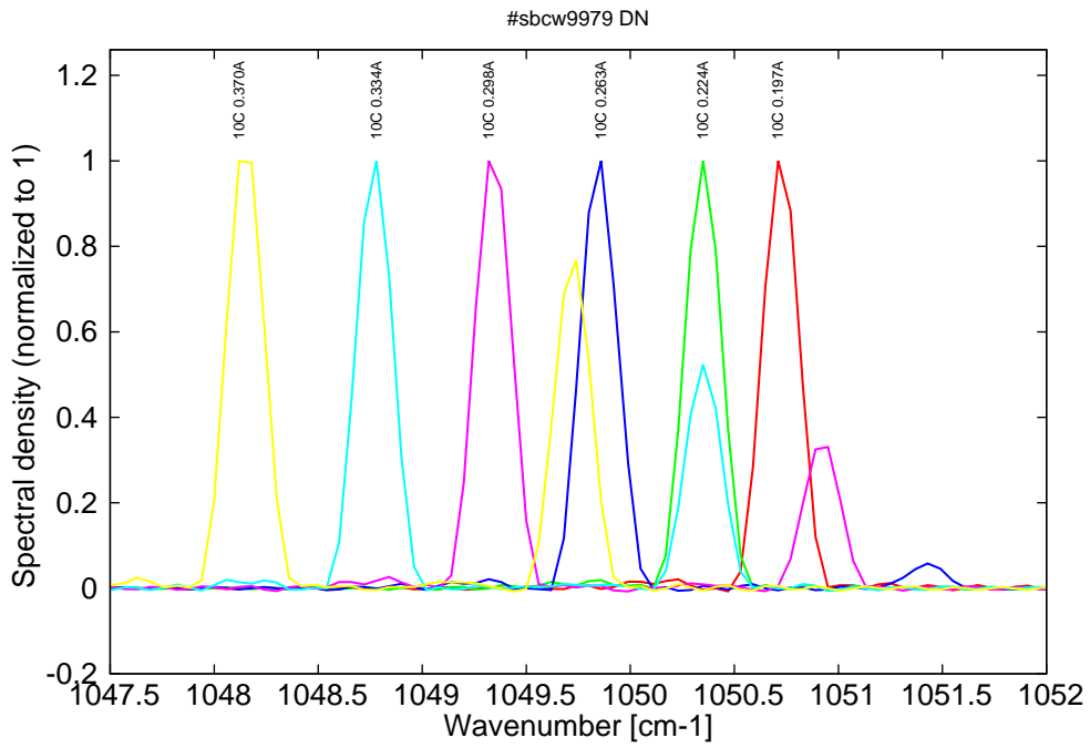
Figure 12: spectra at 10C for various DC currents (monomode up to 0.225A, then becomes bimode)
