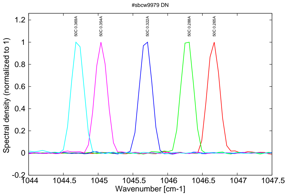
Figure 23: spectra at 50C for various DC currents (monomode range)
