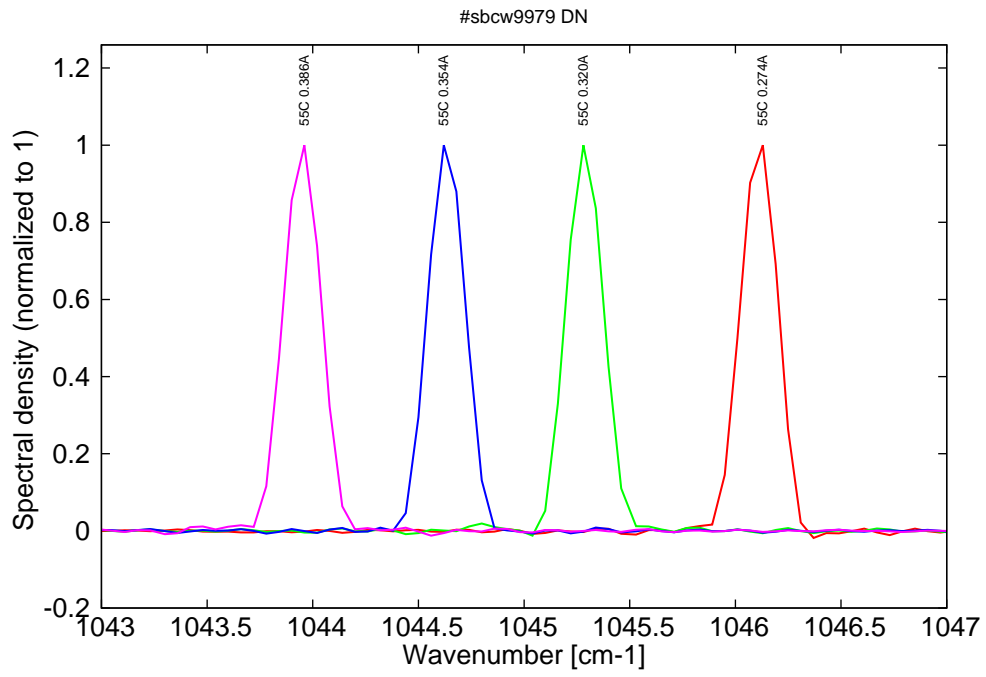
Figure 24: spectra at 55C for various DC currents (all monomode)
