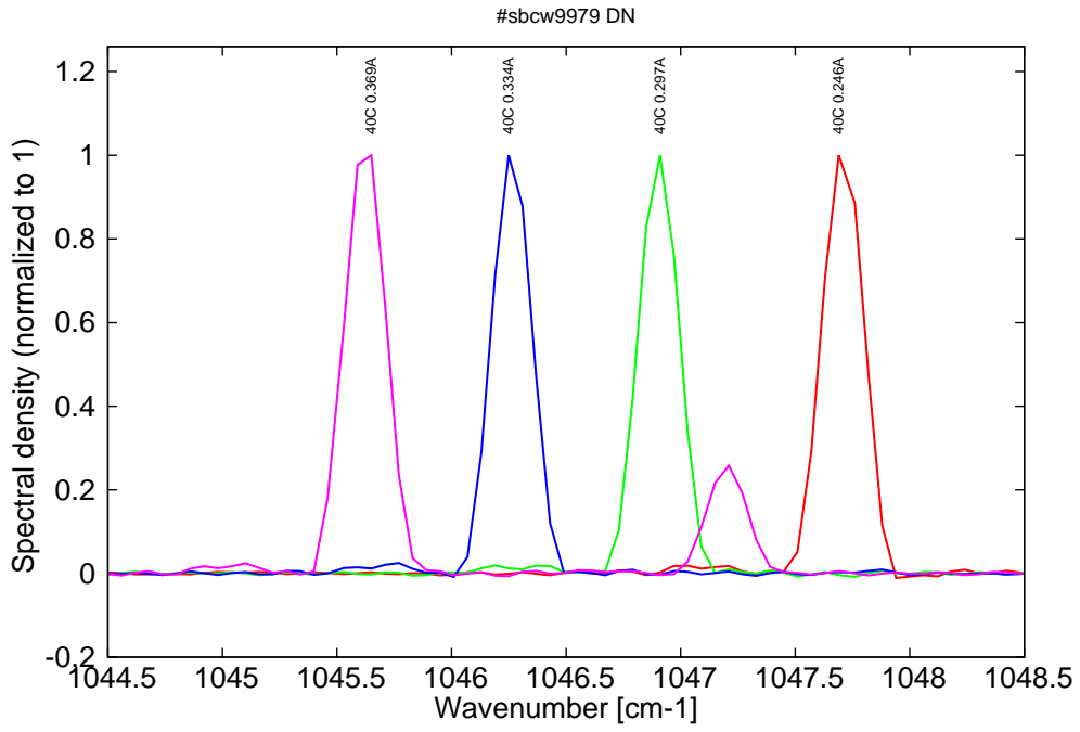
Figure 18: spectra at 40C for various DC currents (monomode up to 0.300A, then becomes bimode)
