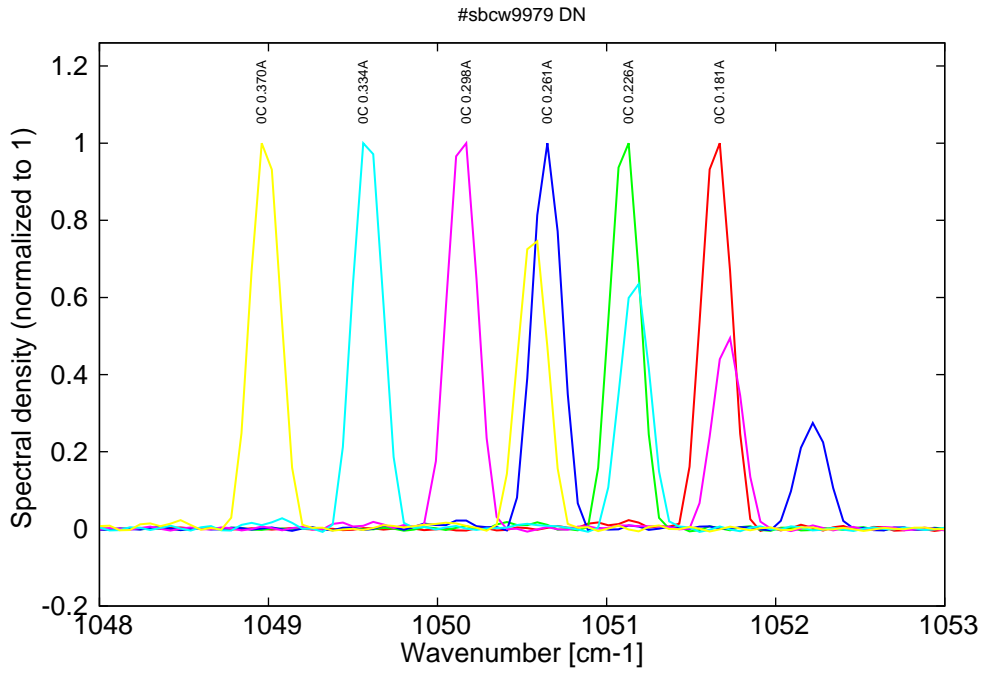
Figure 10: spectra at 0C for various DC currents (monomode up to 0.225A, then becomes bimode)
