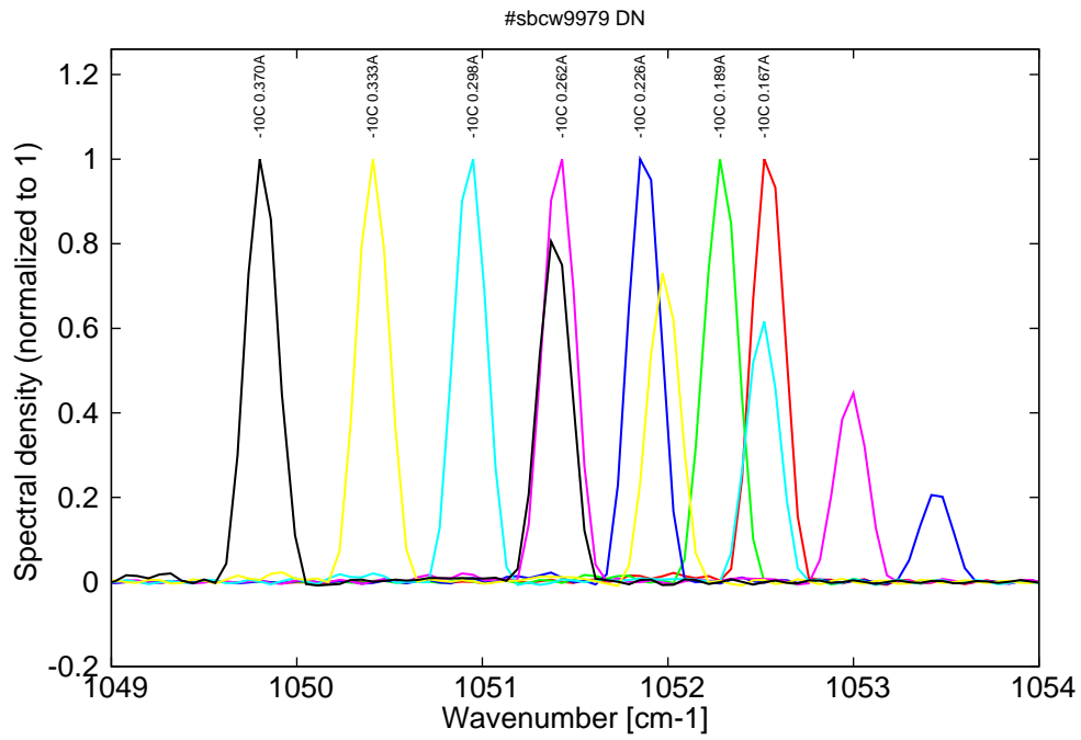
Figure 8: spectra at -10C for various DC currents (monomode up to 0.19A, then becomes bimode)
