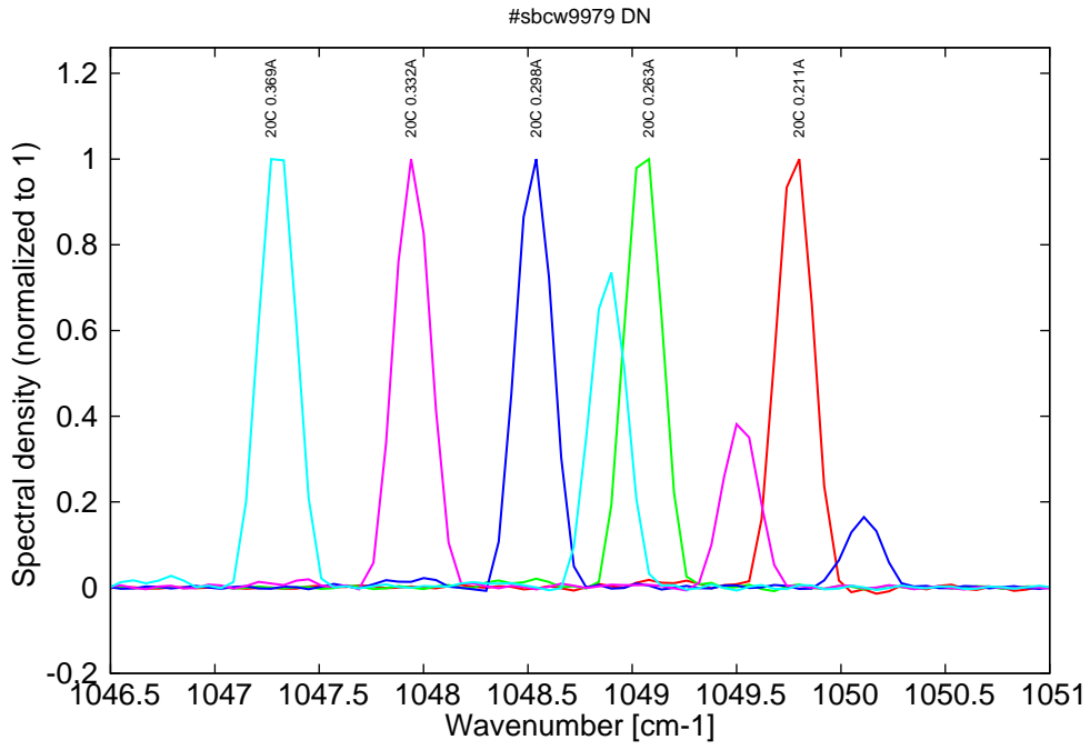
Figure 14: spectra at 20C for various DC currents (monomode up to 0.265A, then becomes bimode)
